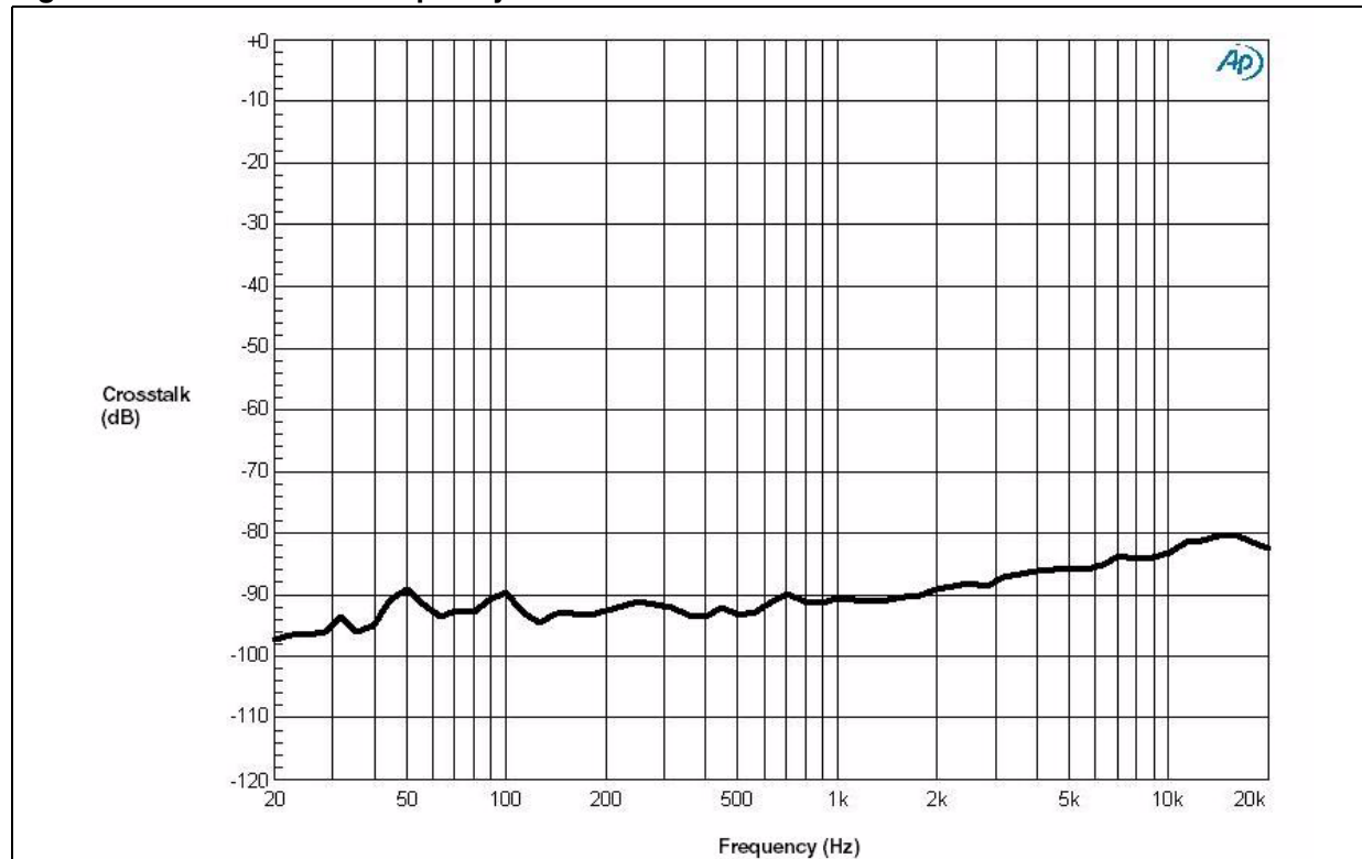
Figure 8. Crosstalk vs. frequency
