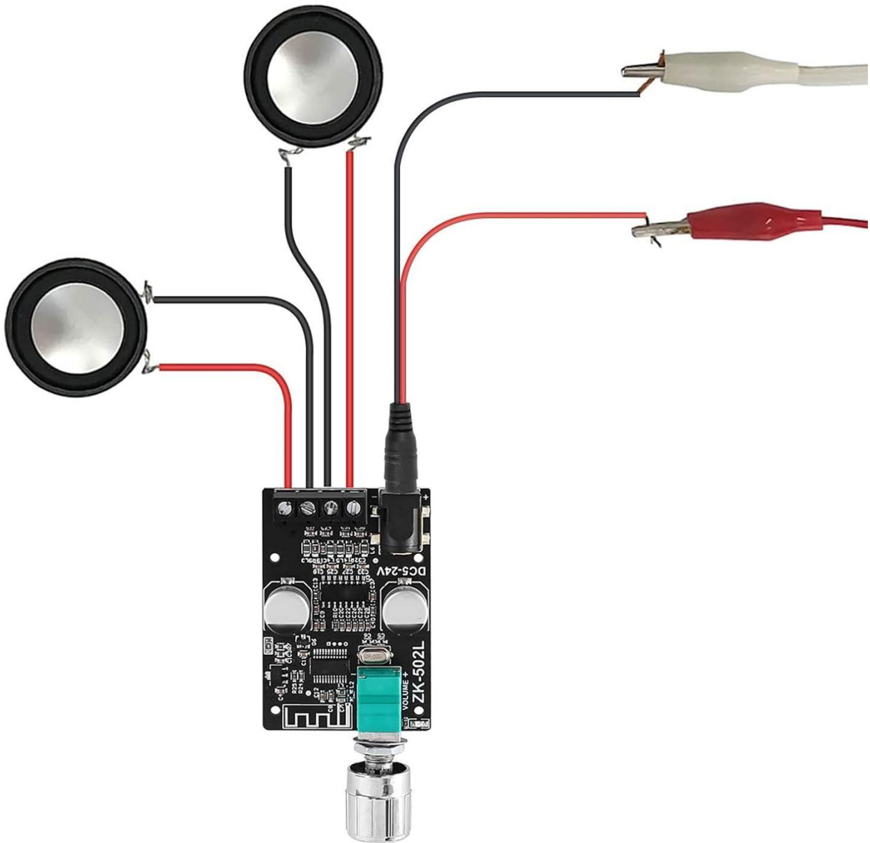
Figure 5: Diagram illustrating the correct connection of speakers and power supply to the ZK-502L amplifier board.
