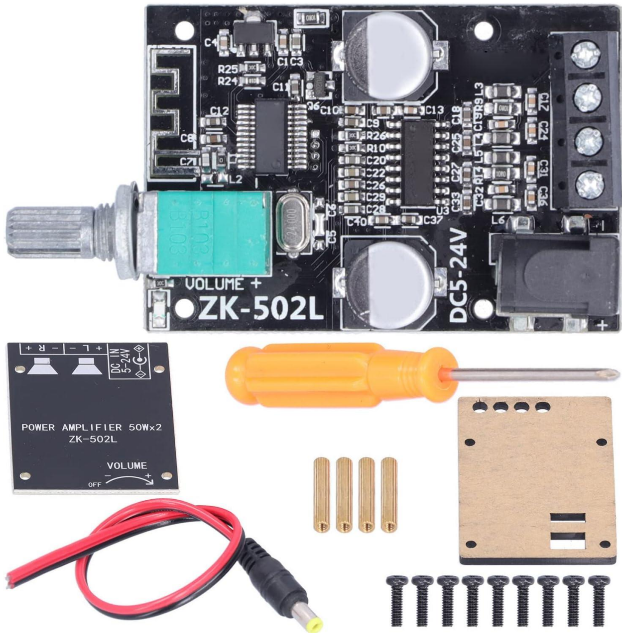
Figure 4: Contents of the ZK-502L amplifier kit, including the board, protective casing, and accessories.
