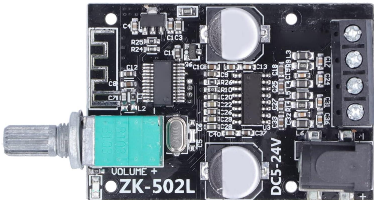
Figure 2: Detailed view of the ZK-502L board highlighting key components and protection features.
