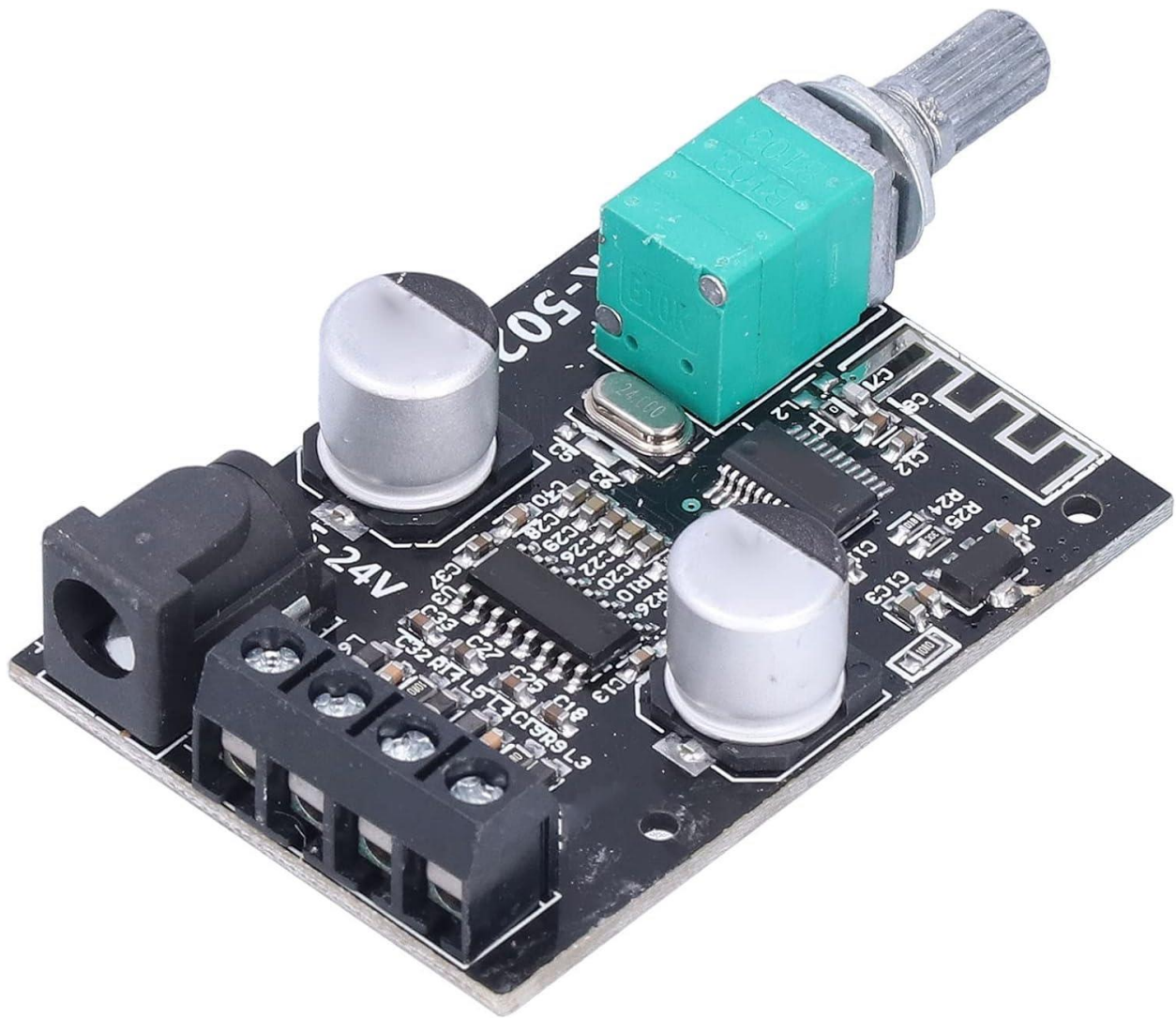
Figure 1: ZK-502L Bluetooth Power Amplifier Board. This image shows the compact design of the amplifier board with its various components, including the volume potentiometer, power input, and speaker terminals.
