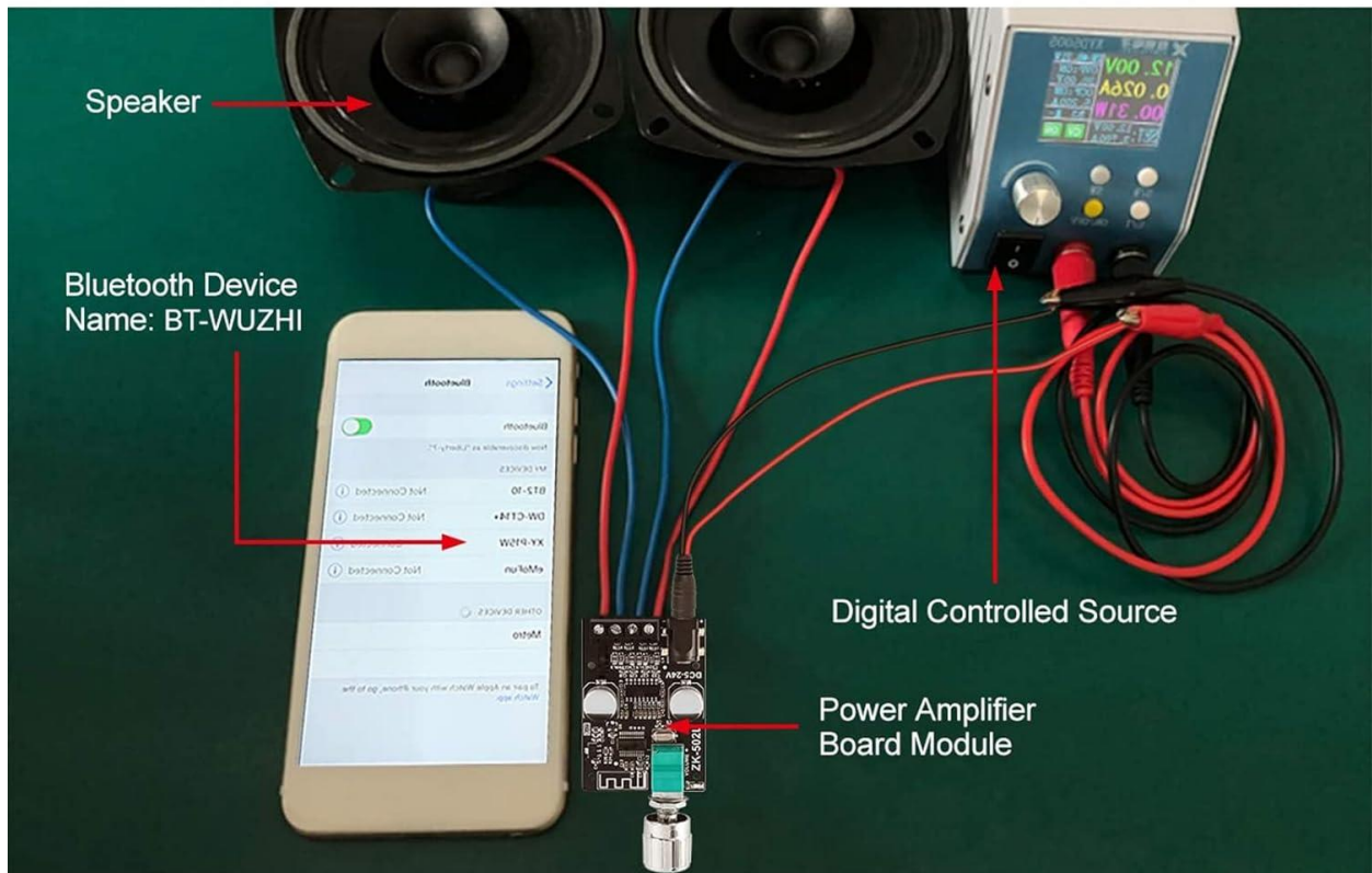
Figure 6: Visual guide demonstrating the steps for connecting and using the ZK-502L amplifier board with a mobile device and speakers.
